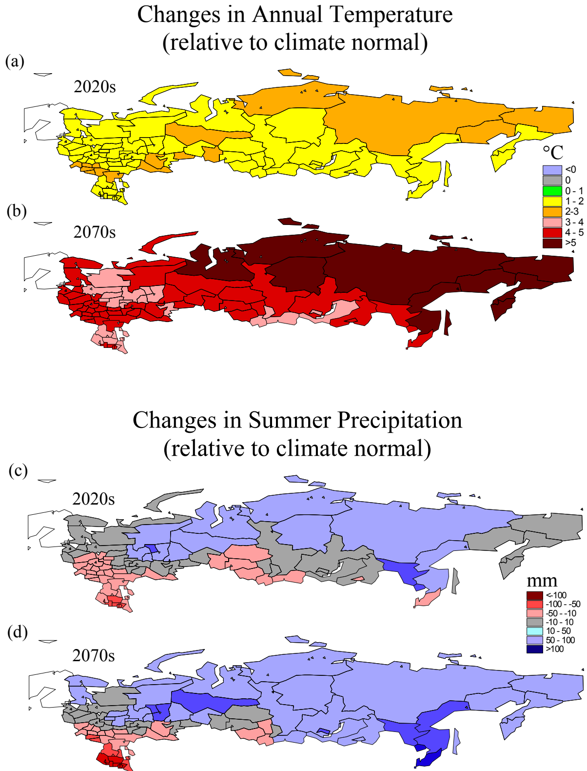
Figure 2: Changes in climate (relative to climate normal) for the A2 scenario computed by the HADC3 model: (a) annual surface temperature for 2020s, (b) for 2070s, (c) summer precipitation (July, August, September) for 2020s, (d) for 2070s. Note that temperature changes are annual averages and precipitation changes are summer averages.
