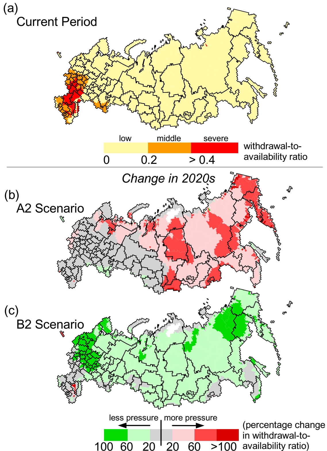
Figure 4: Pressure on water resources as indicated by the withdrawals-to-availability ratio (wta) computed by the WaterGAP model with climate scenarios from HADCM3: (a) current wta, (b) change in wta in 2020s under the A2 scenario, (c) change in wta under the B2 scenario.
